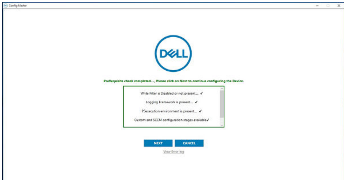
Figure 4. Config Master
