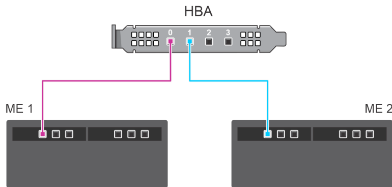
Figure 13. Single Path Configuration: Cabling of HBA355e Adapter with ME484 Enclosures
