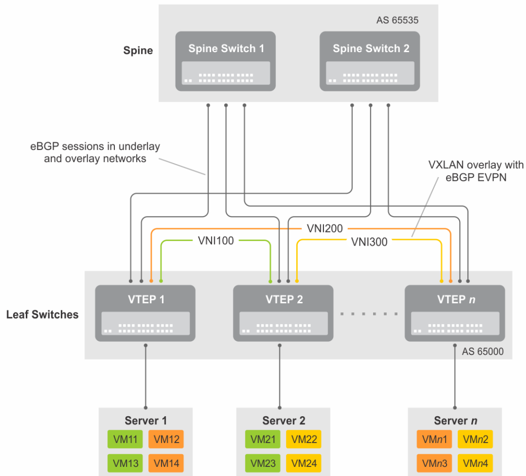
Figure 13. BGP EVPN topology
